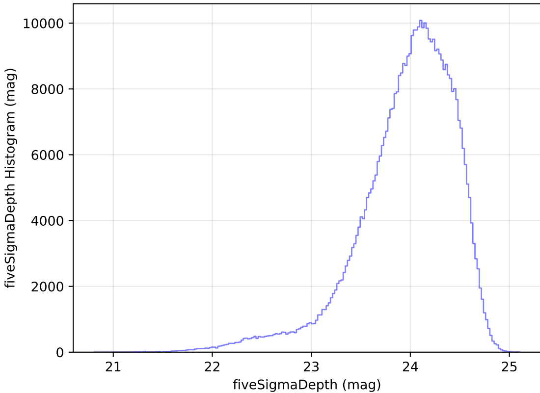
reweight_bulge_v3.3_10yrs r: fiveSigmaDepth Histogram
