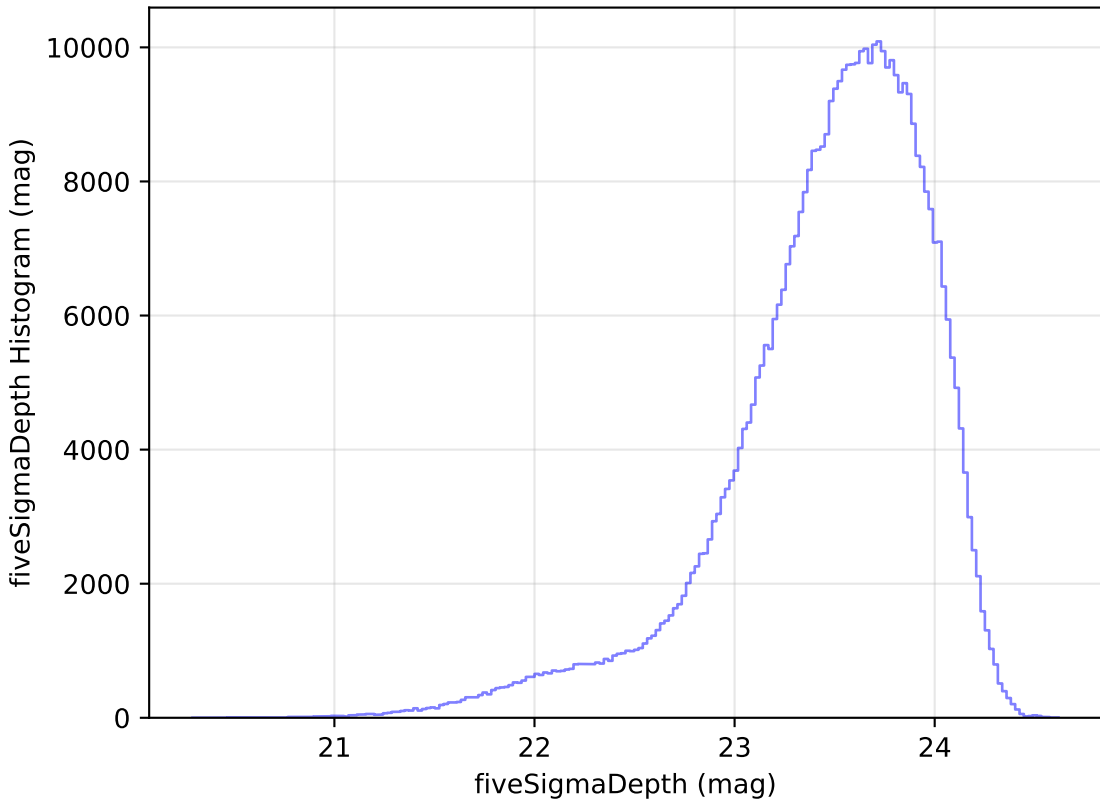
reweight_bulge_v3.3_10yrs i: fiveSigmaDepth Histogram
