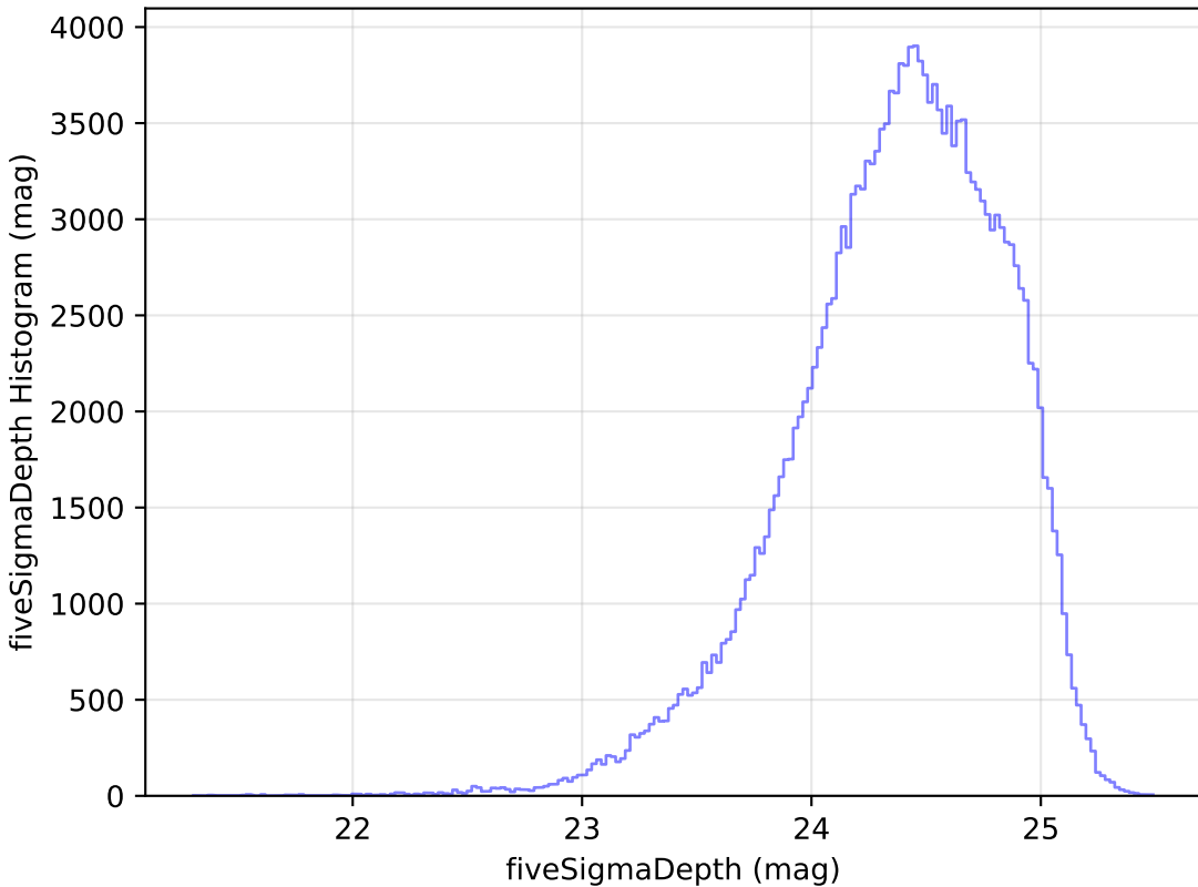
reweight_bulge_v3.3_10yrs g: fiveSigmaDepth Histogram
