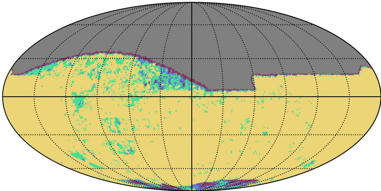
reweight_bulge_v3.3_10yrs z band: YearCoverage night
