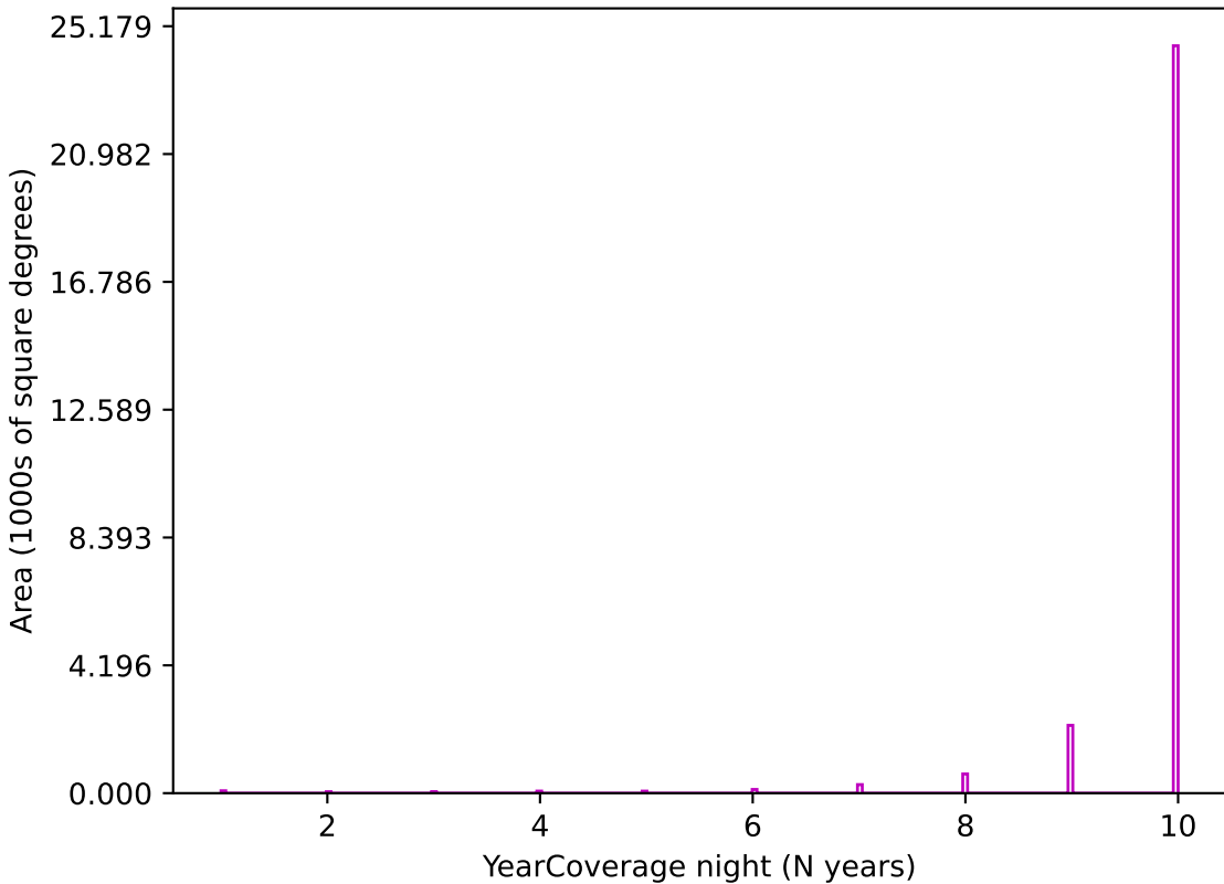
reweight_bulge_v3.3_10yrs z band: YearCoverage night
