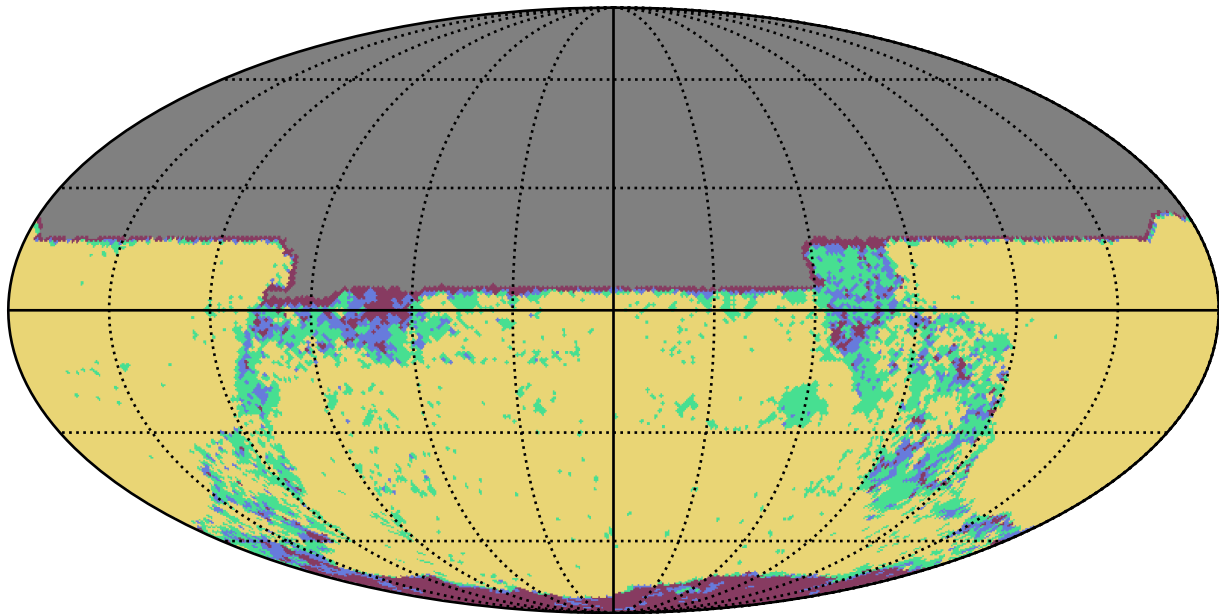
reweight_bulge_v3.3_10yrs y band: YearCoverage night
