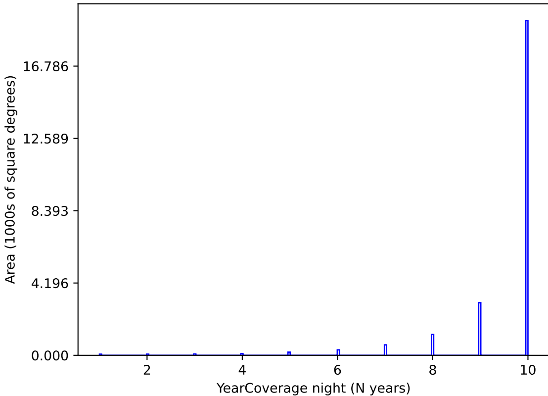
reweight_bulge_v3.3_10yrs y band: YearCoverage night
