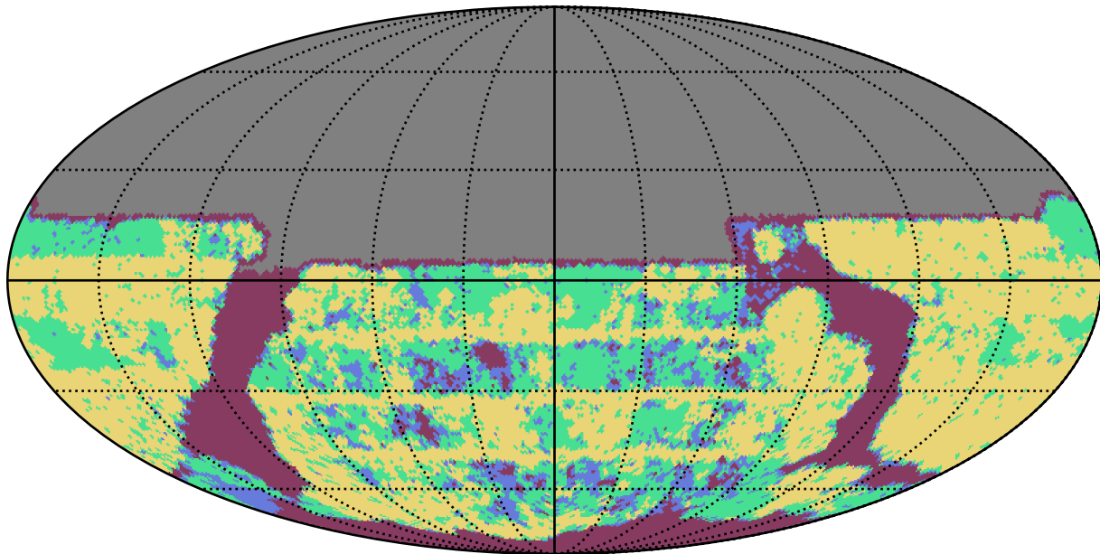
reweight_bulge_v3.3_10yrs u band: YearCoverage night
