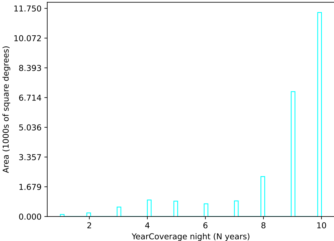
reweight_bulge_v3.3_10yrs u band: YearCoverage night
