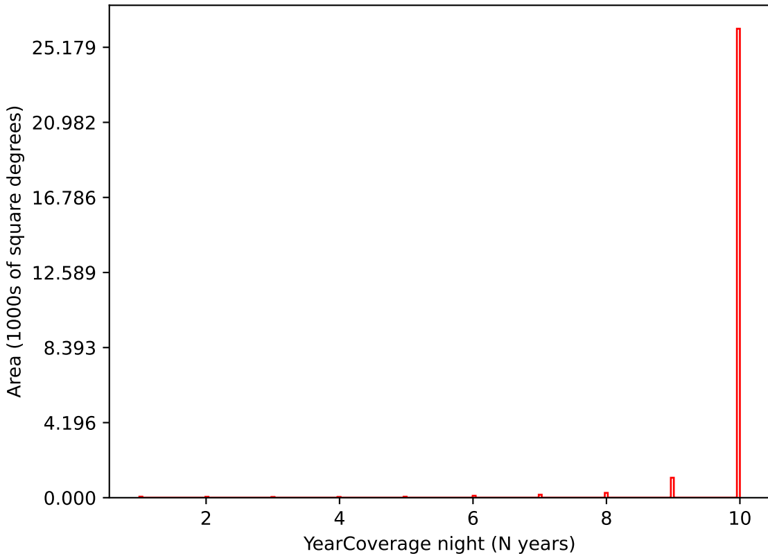
reweight_bulge_v3.3_10yrs i band: YearCoverage night
