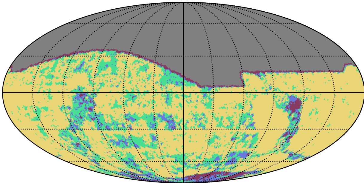
reweight_bulge_v3.3_10yrs g band: YearCoverage night
