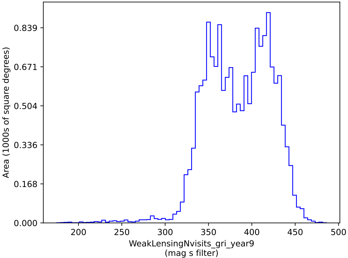
reweight_bulge_v3.3_10yrs gri band non-DD: WeakLensingNvisits_gri_year9
