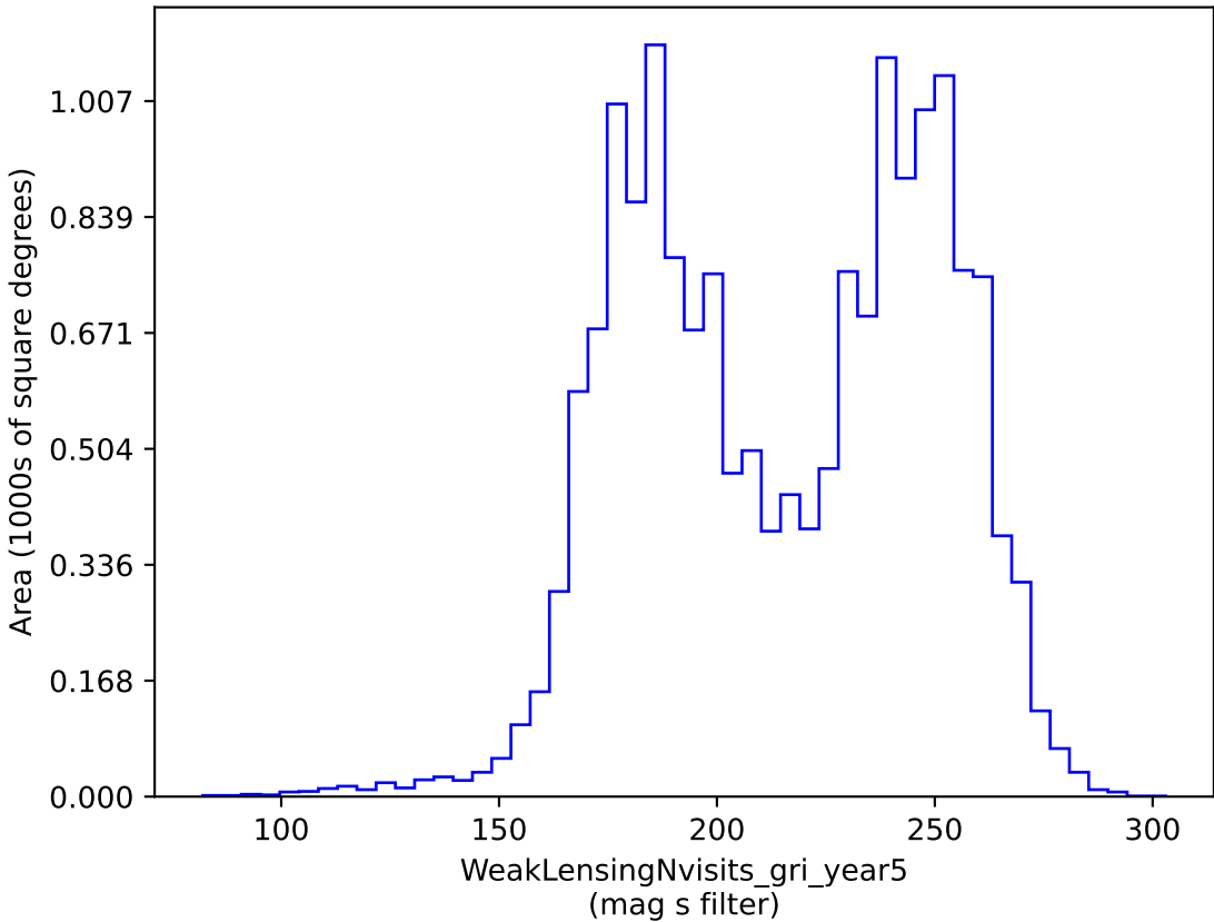
reweight_bulge_v3.3_10yrs gri band non-DD: WeakLensingNvisits_gri_year5
