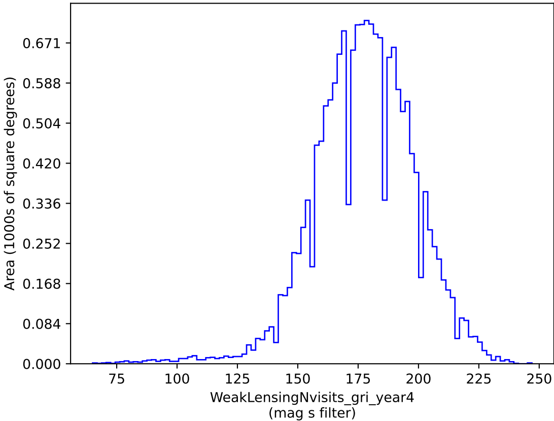
reweight_bulge_v3.3_10yrs gri band non-DD: WeakLensingNvisits_gri_year4
