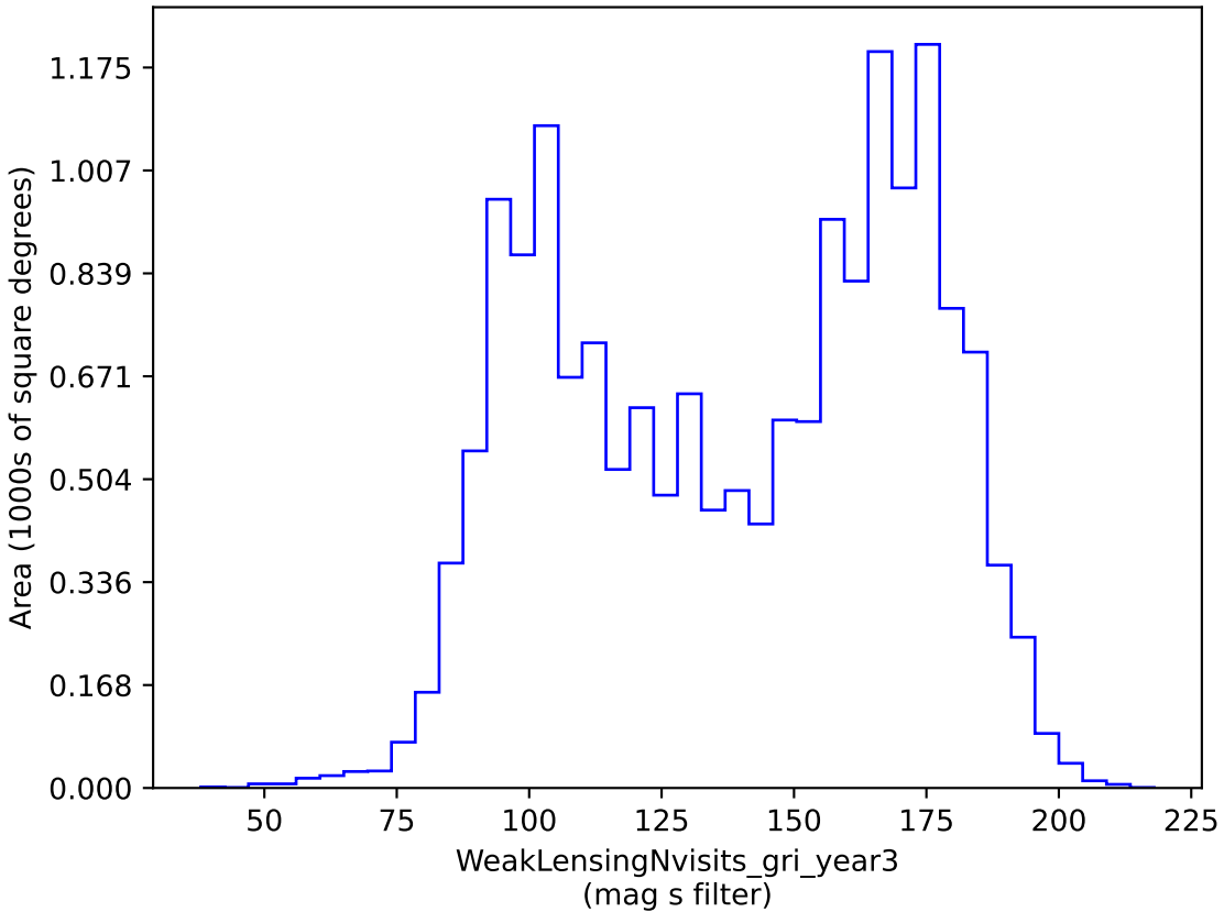
reweight_bulge_v3.3_10yrs gri band non-DD: WeakLensingNvisits_gri_year3
