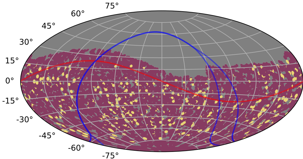
reweight_bulge_v3.3_10yrs : TDEsPopMetric_some_color
