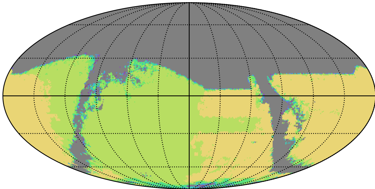
reweight_bulge_v3.3_10yrs : TDC_campaign
