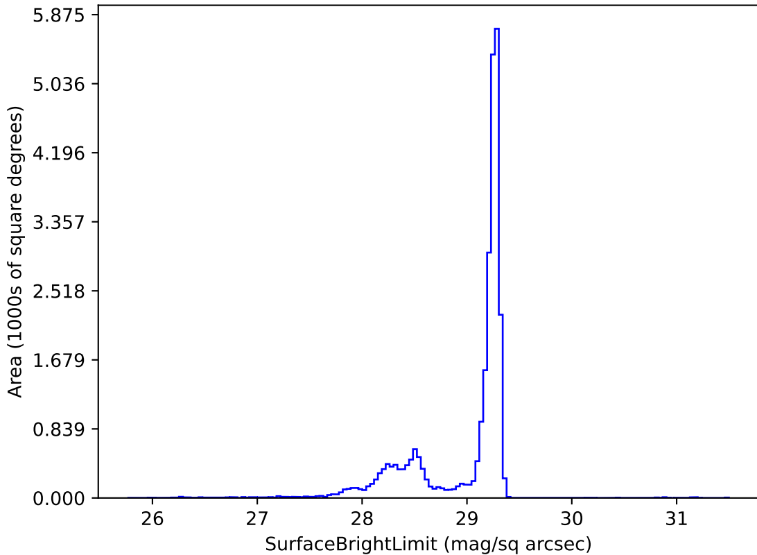
reweight_bulge_v3.3_10yrs z: SurfaceBrightLimit
