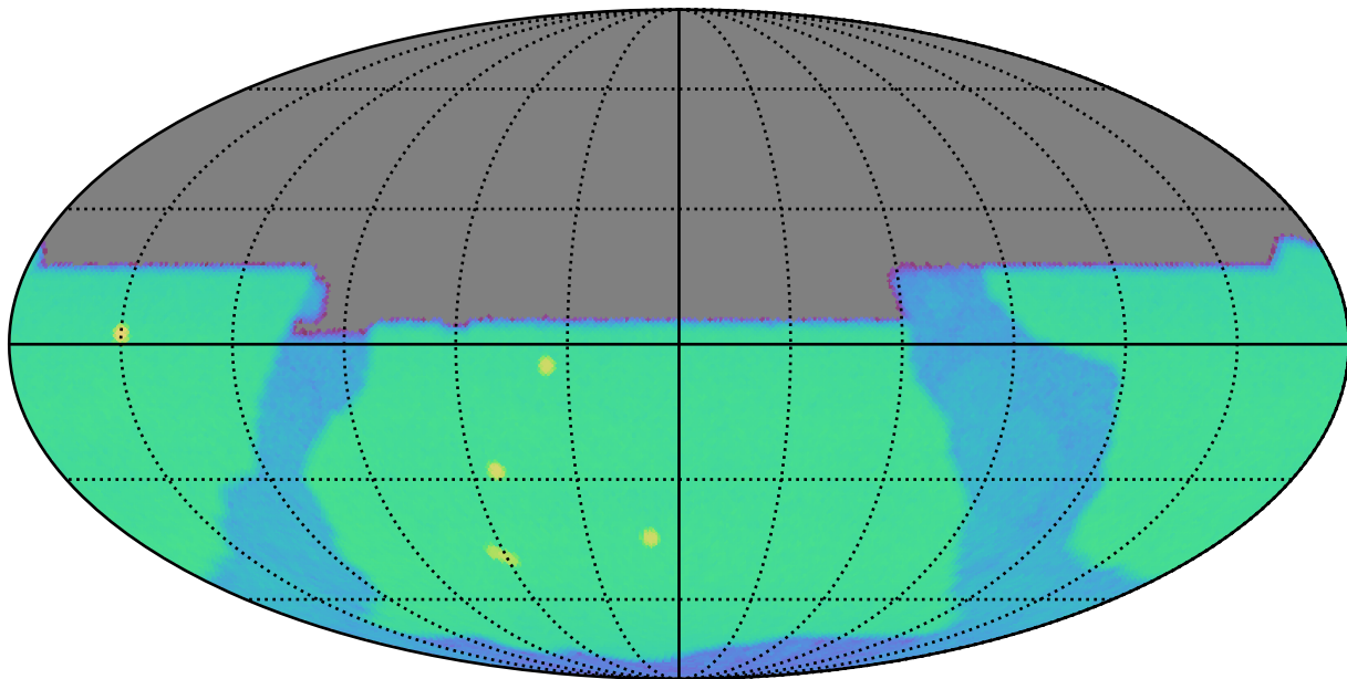
reweight_bulge_v3.3_10yrs y: SurfaceBrightLimit
