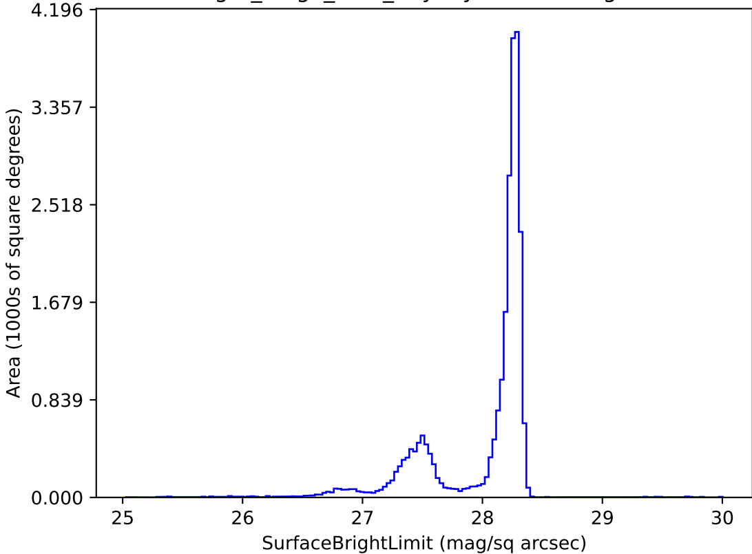
reweight_bulge_v3.3_10yrs y: SurfaceBrightLimit
