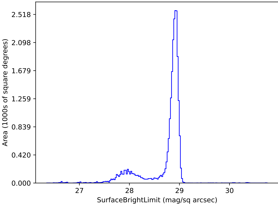
reweight_bulge_v3.3_10yrs u: SurfaceBrightLimit
