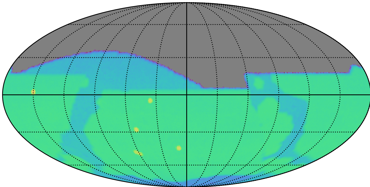
reweight_bulge_v3.3_10yrs r: SurfaceBrightLimit
