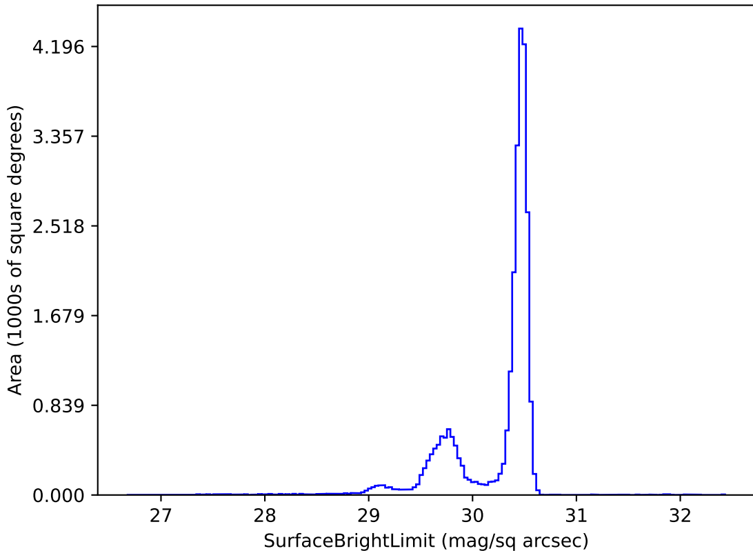
reweight_bulge_v3.3_10yrs r: SurfaceBrightLimit
