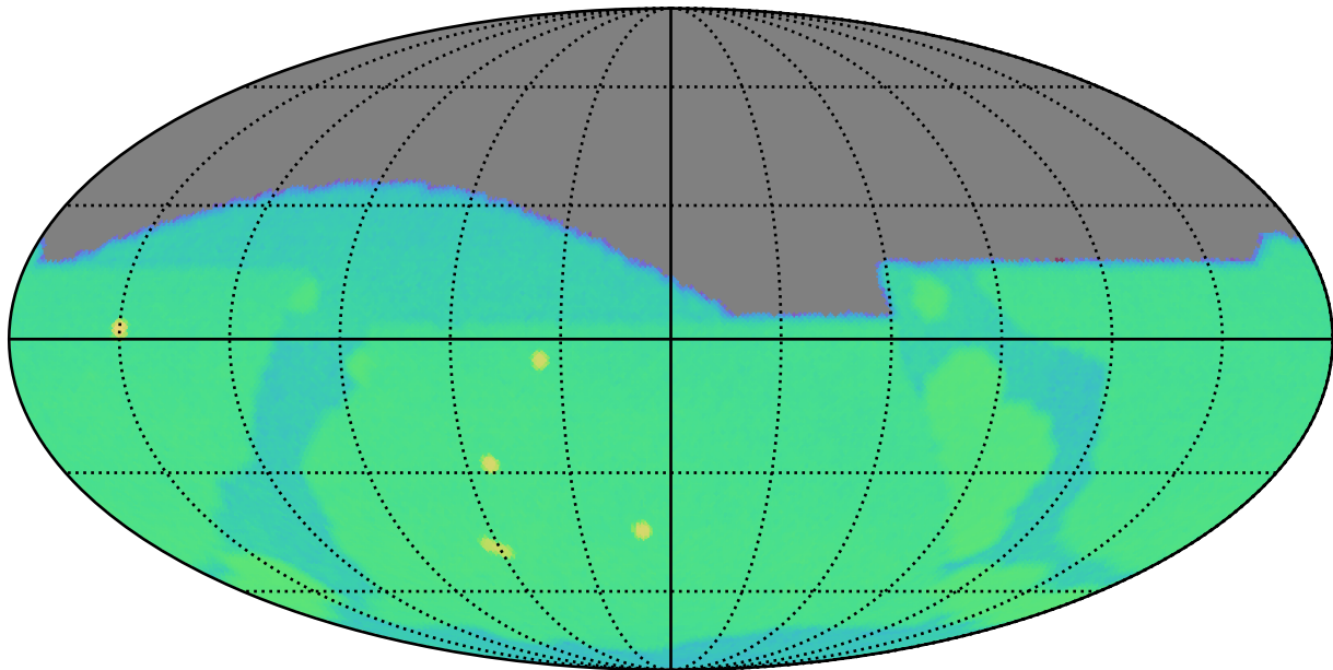
reweight_bulge_v3.3_10yrs g: SurfaceBrightLimit
