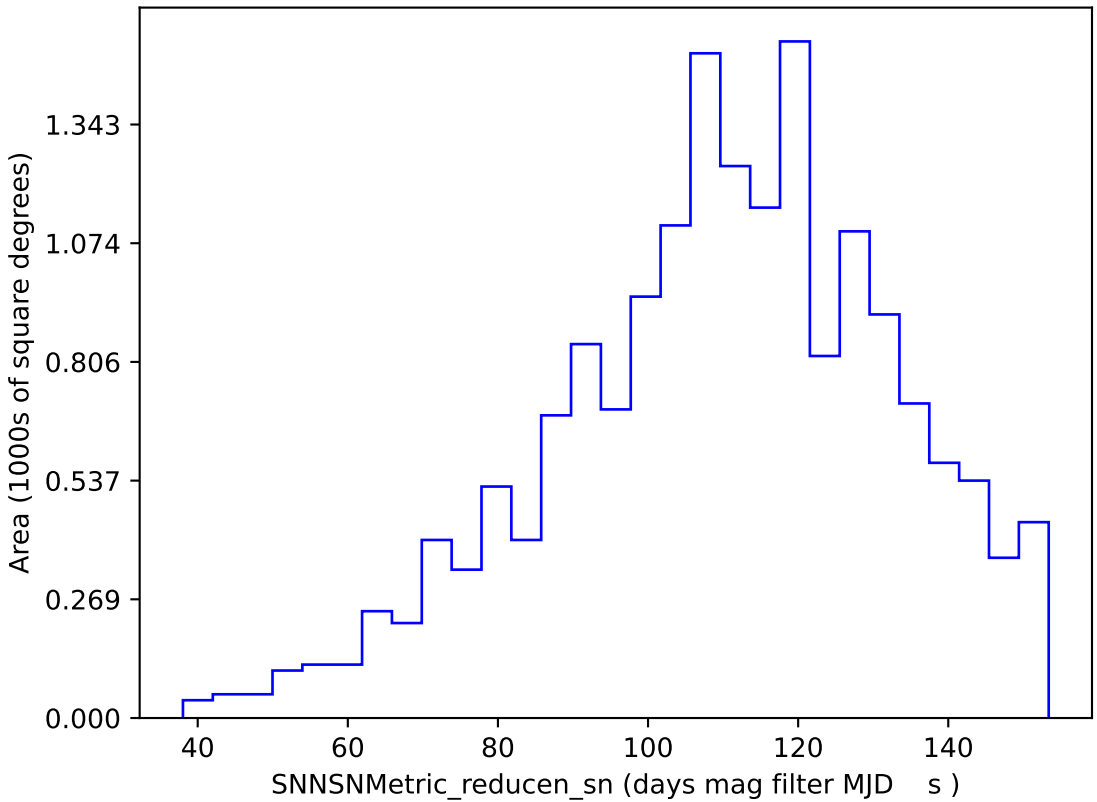
reweight_bulge_v3.3_10yrs DDF excluded: SNNSNMetric_reducen_sn
