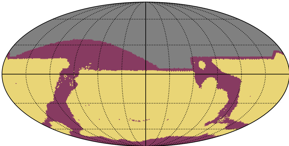
reweight_bulge_v3.3_10yrs : RapidRevisits
