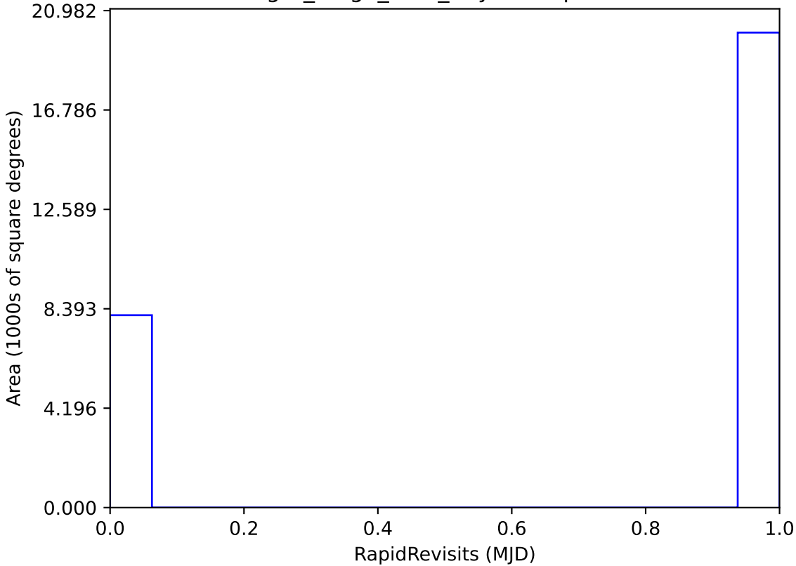
reweight_bulge_v3.3_10yrs : RapidRevisits
