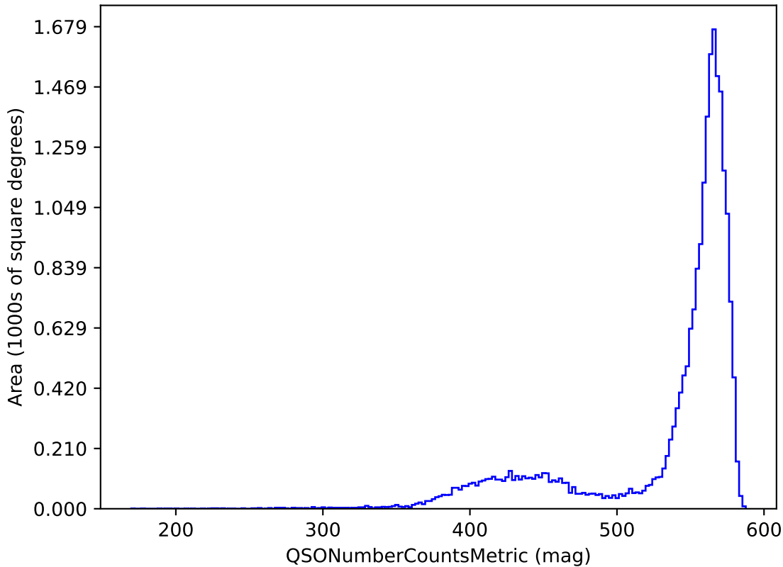
reweight_bulge_v3.3_10yrs y band and non-DD: QSONumberCountsMetric
