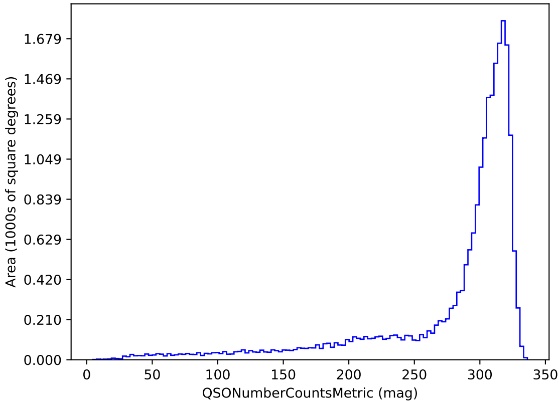
reweight_bulge_v3.3_10yrs u band and non-DD: QSONumberCountsMetric
