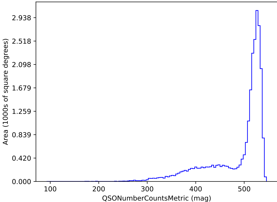
reweight_bulge_v3.3_10yrs r band and non-DD: QSONumberCountsMetric
