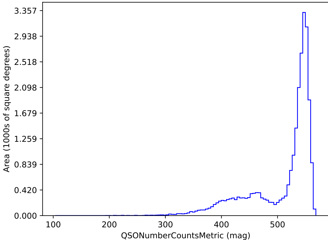
reweight_bulge_v3.3_10yrs i band and non-DD: QSONumberCountsMetric
