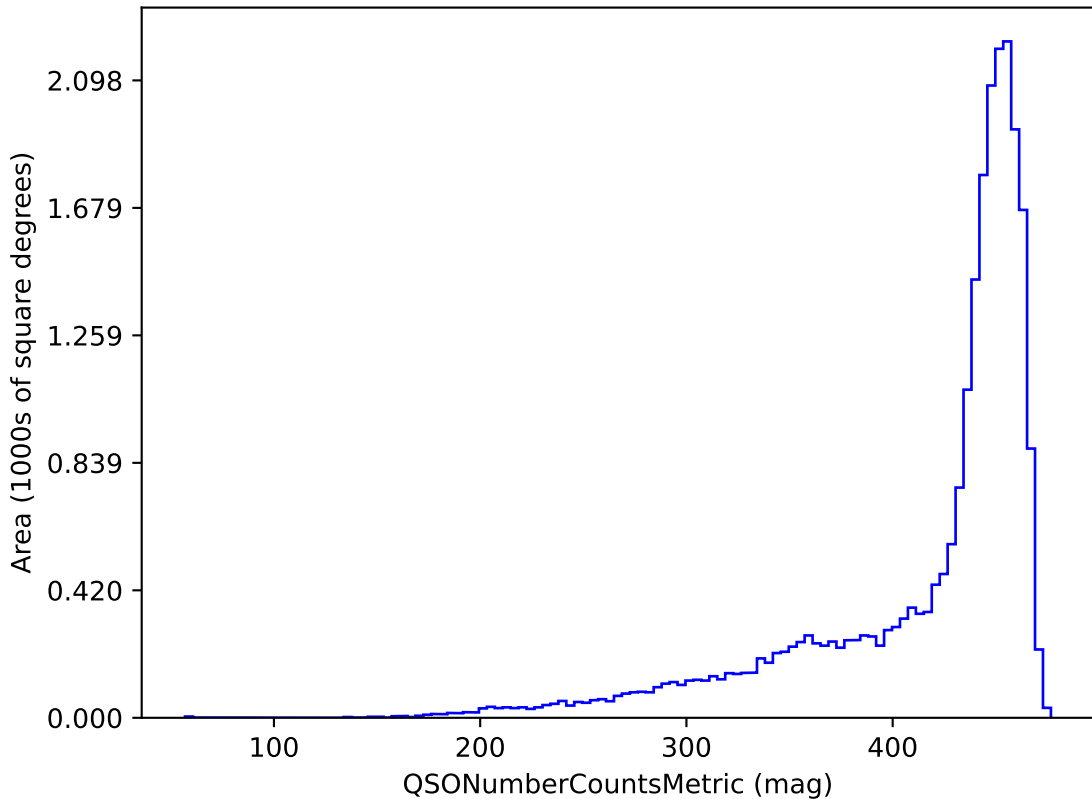
reweight_bulge_v3.3_10yrs g band and non-DD: QSONumberCountsMetric
