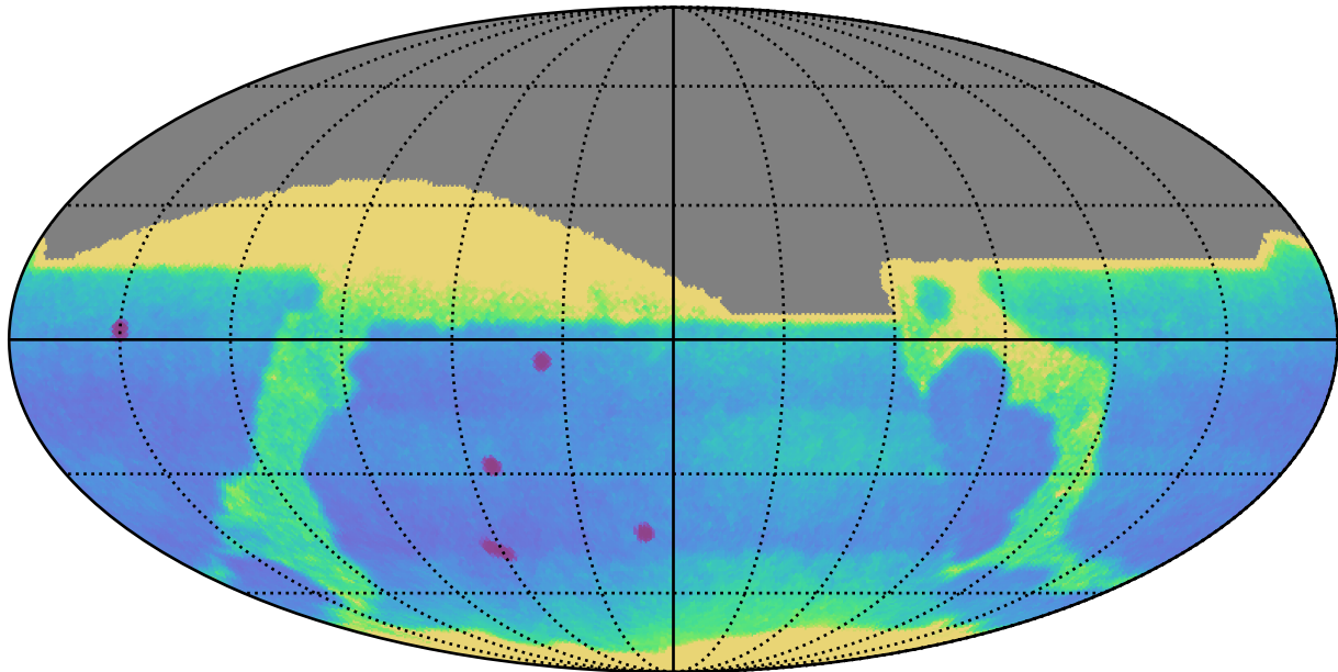
reweight_bulge_v3.3_10yrs : Proper Motion Uncert @ 24.0
