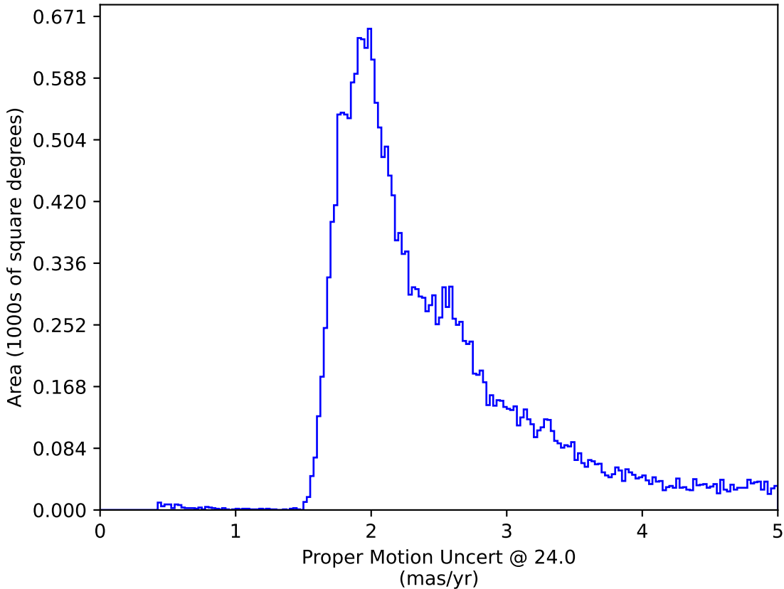
reweight_bulge_v3.3_10yrs : Proper Motion Uncert @ 24.0
