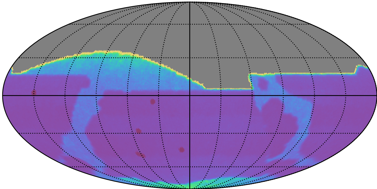
reweight_bulge_v3.3_10yrs : Proper Motion Uncert @ 20.5
