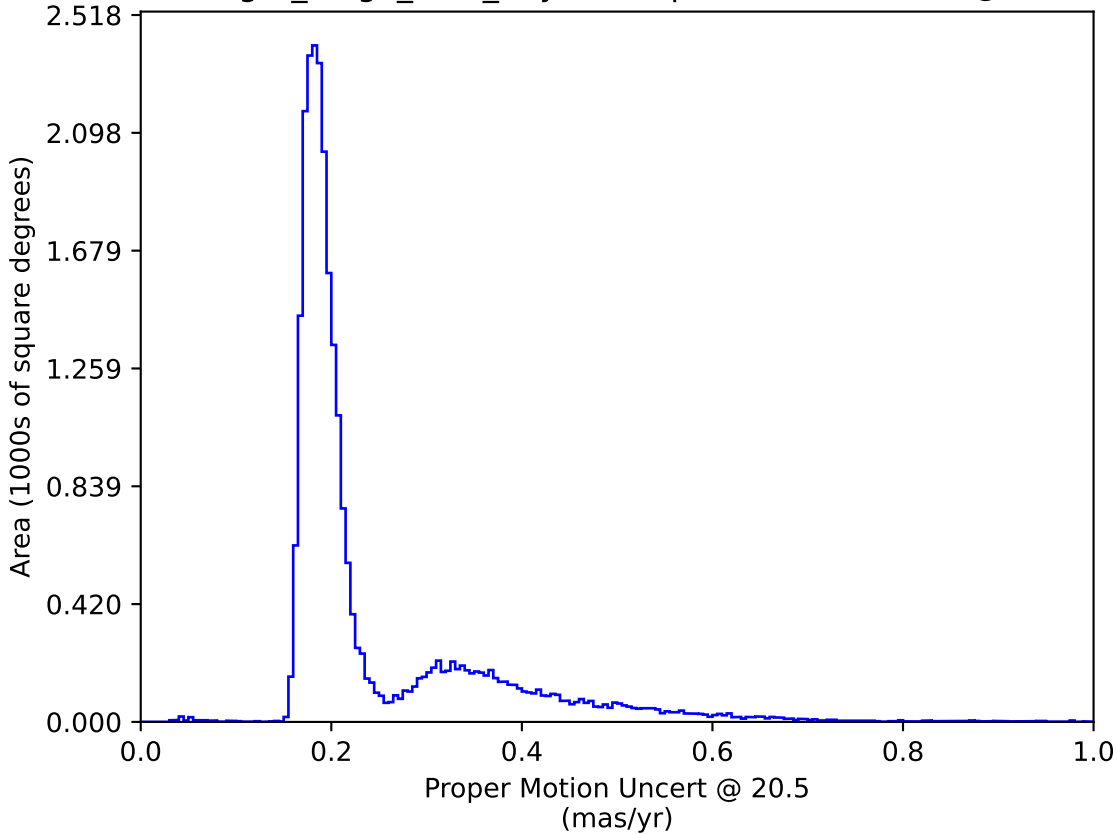
reweight_bulge_v3.3_10yrs : Proper Motion Uncert @ 20.5
