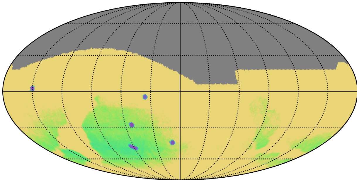
reweight_bulge_v3.3_10yrs : Parallax Uncert @ 22.4
