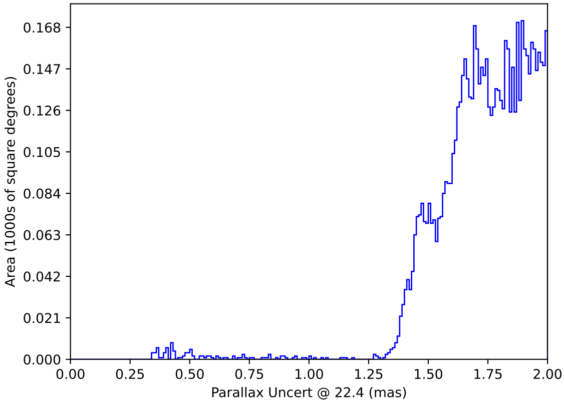
reweight_bulge_v3.3_10yrs : Parallax Uncert @ 22.4
