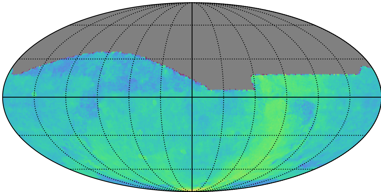
reweight_bulge_v3.3_10yrs : Parallax Coverage @ 24.0
