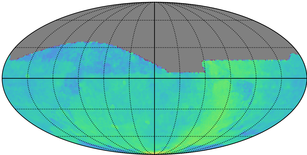
reweight_bulge_v3.3_10yrs : Parallax Coverage @ 22.4
