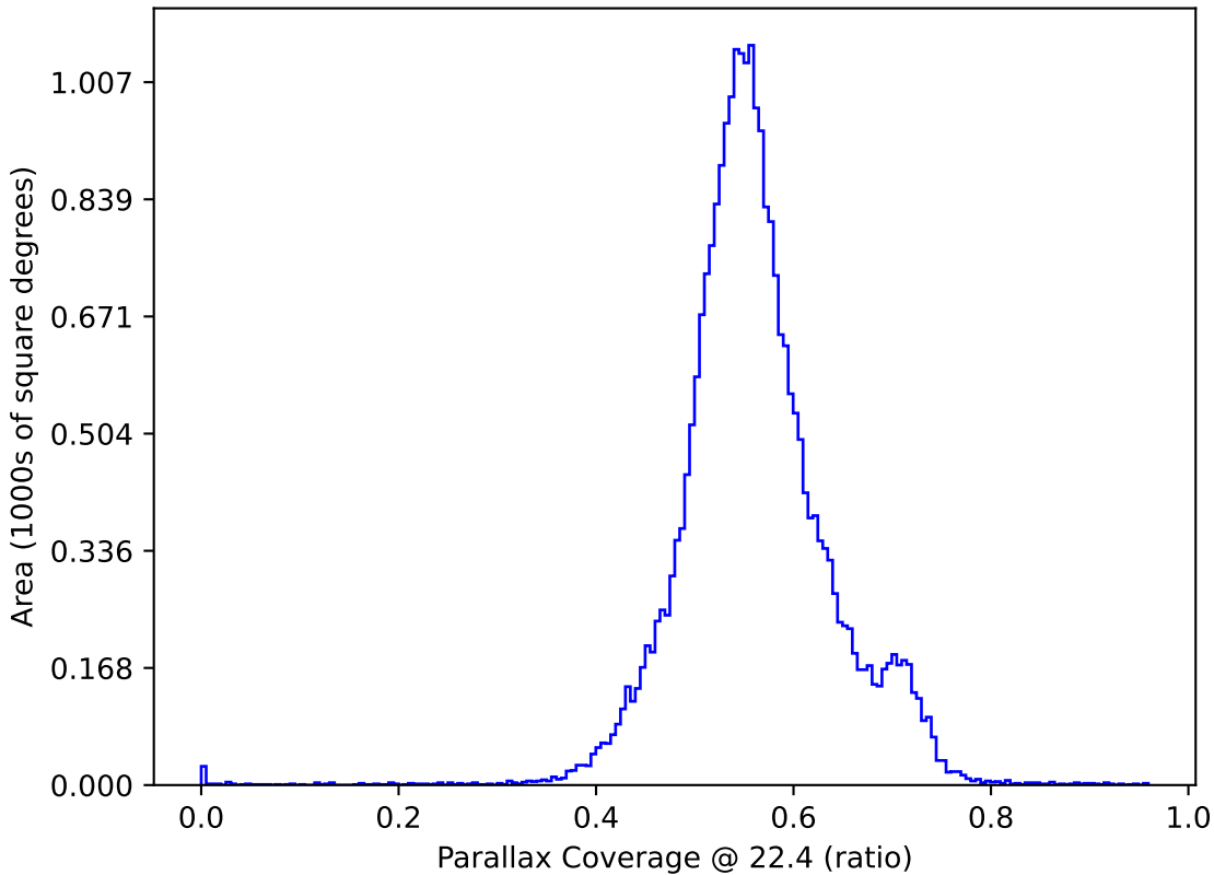
reweight_bulge_v3.3_10yrs : Parallax Coverage @ 22.4
