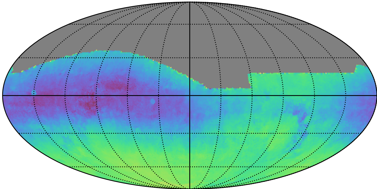
reweight_bulge_v3.3_10yrs : Parallax-DCR degeneracy @ 24.0
