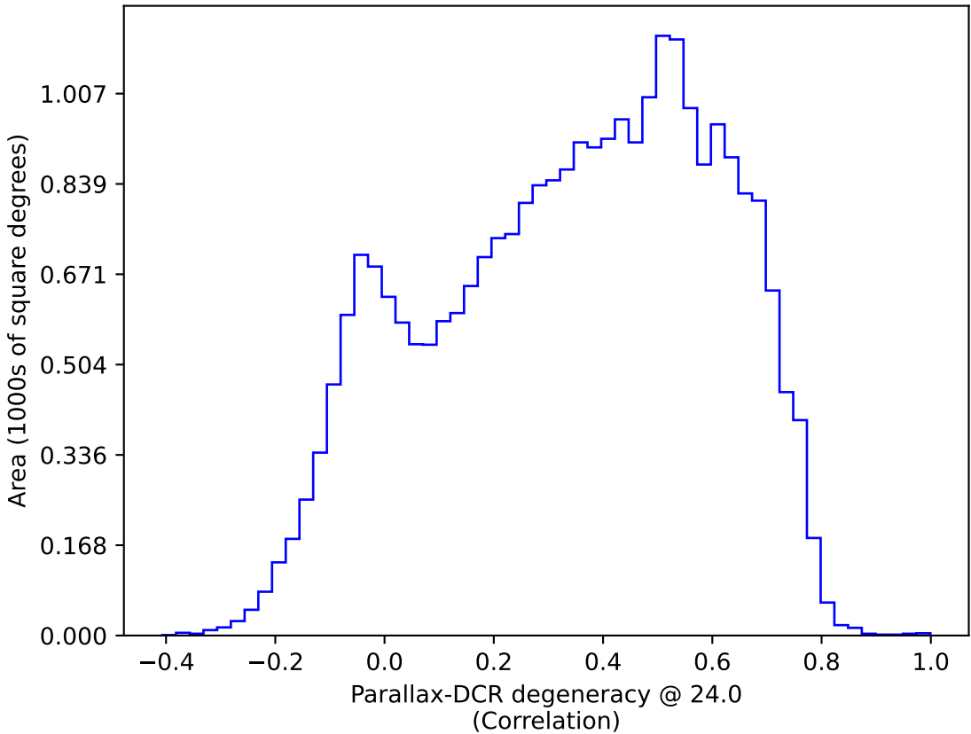
reweight_bulge_v3.3_10yrs : Parallax-DCR degeneracy @ 24.0
