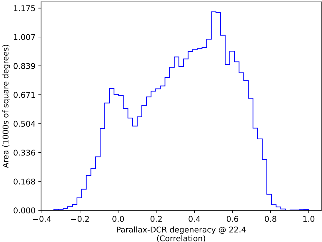
reweight_bulge_v3.3_10yrs : Parallax-DCR degeneracy @ 22.4
