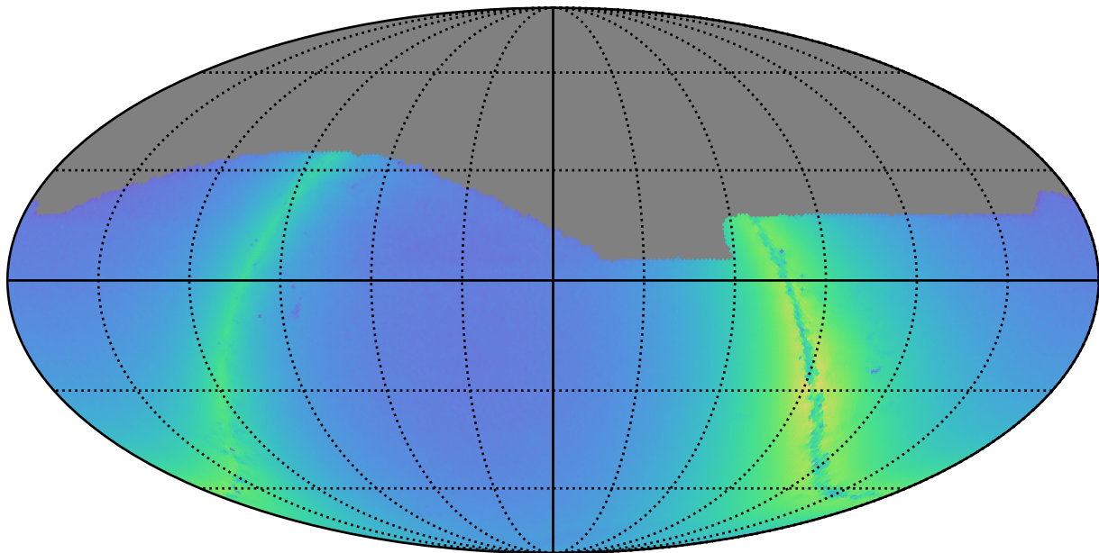
reweight_bulge_v3.3_10yrs z: Nstars_no_crowding
