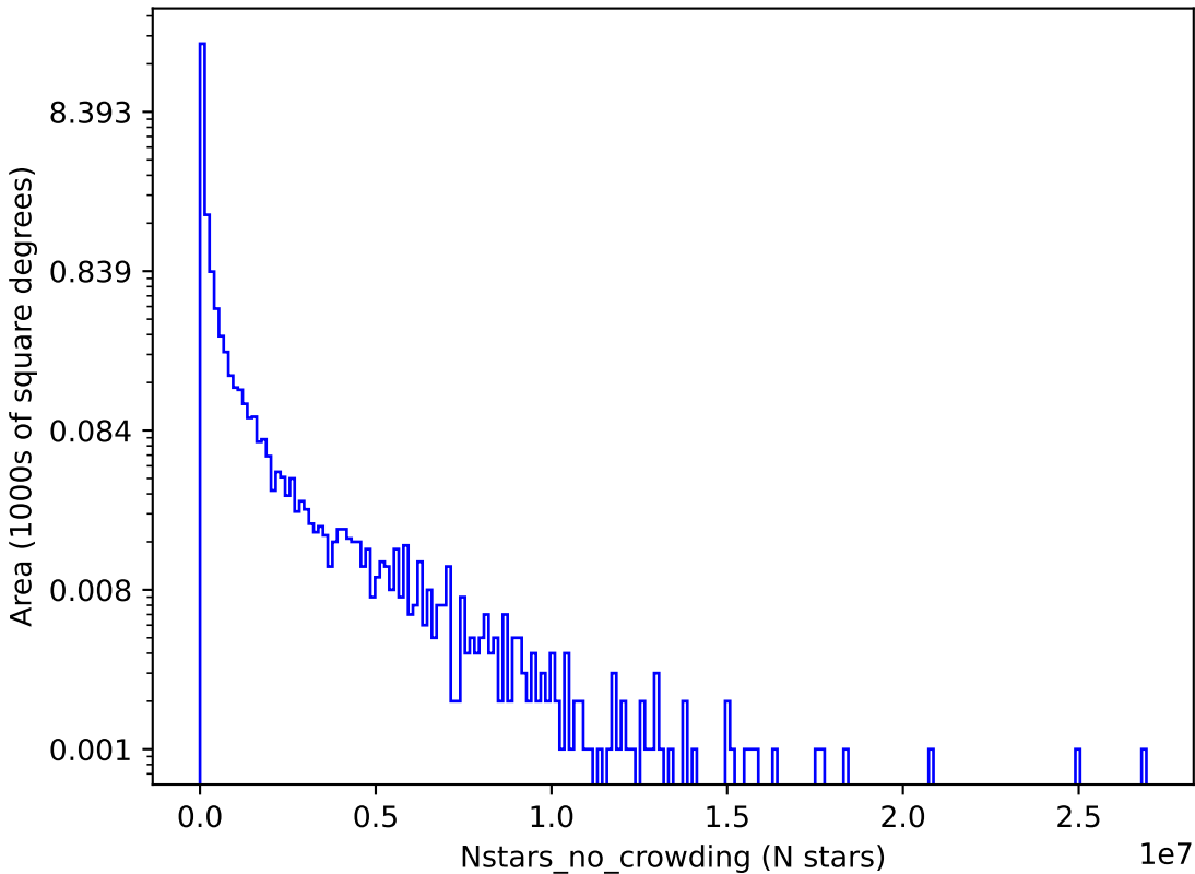
reweight_bulge_v3.3_10yrs z: Nstars_no_crowding
