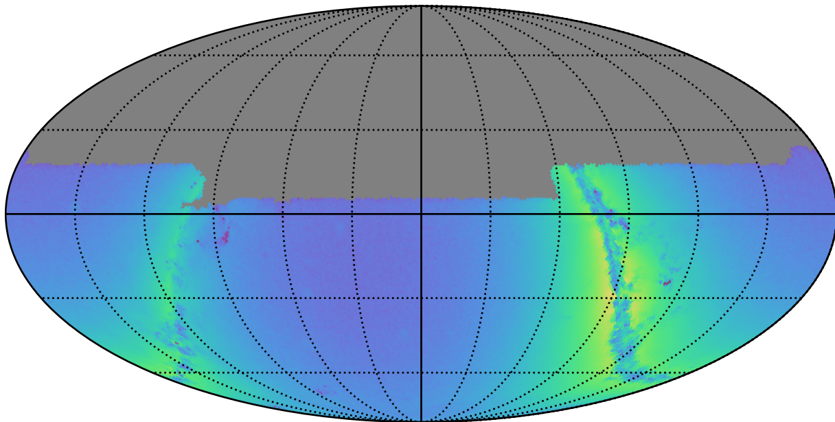
reweight_bulge_v3.3_10yrs u: Nstars_no_crowding
