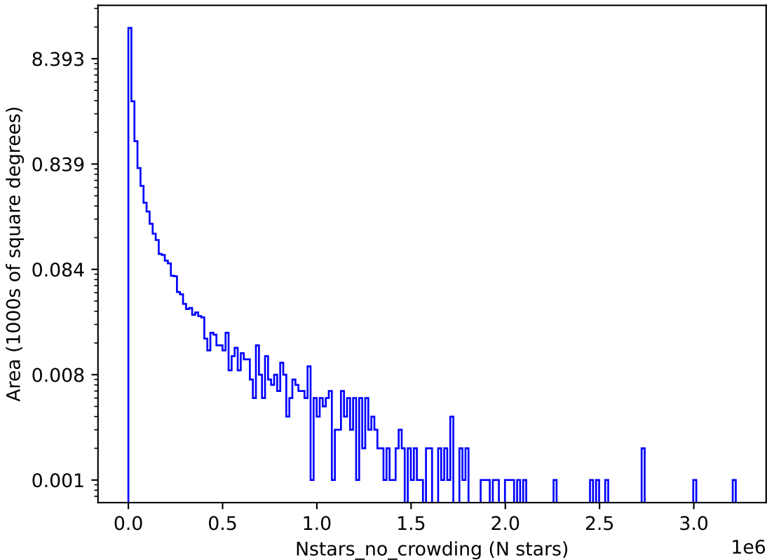
reweight_bulge_v3.3_10yrs u: Nstars_no_crowding
