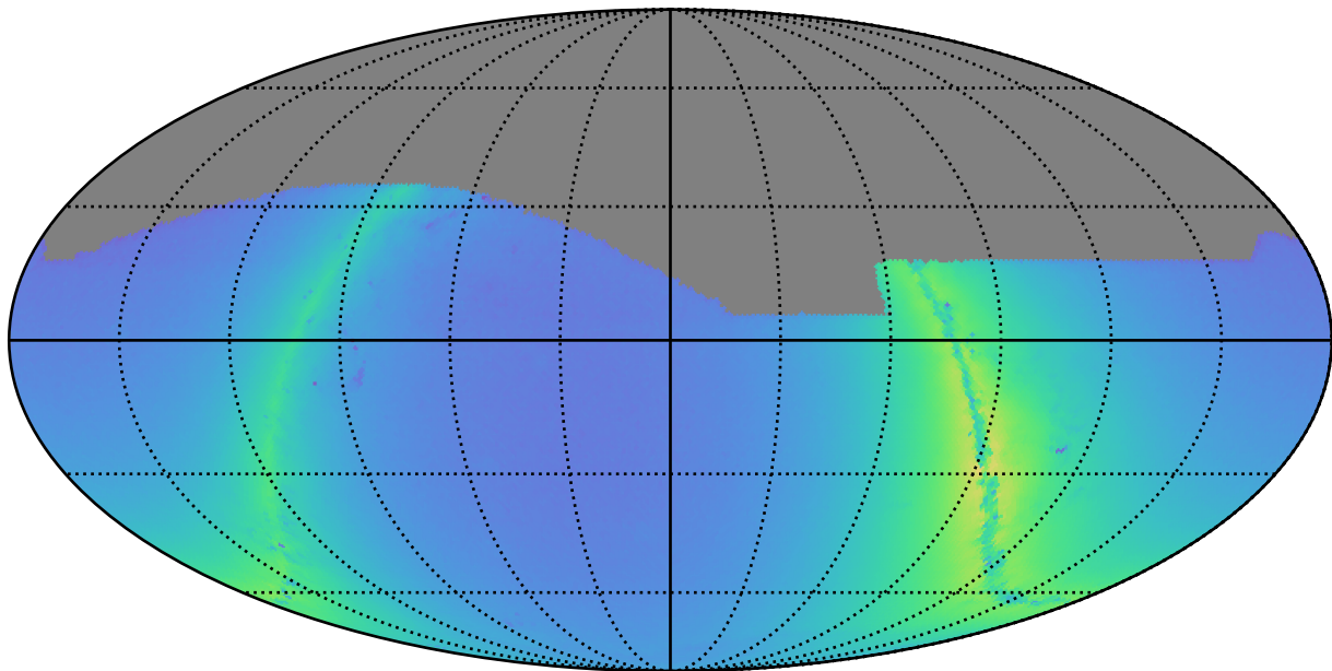
reweight_bulge_v3.3_10yrs r: Nstars_no_crowding
