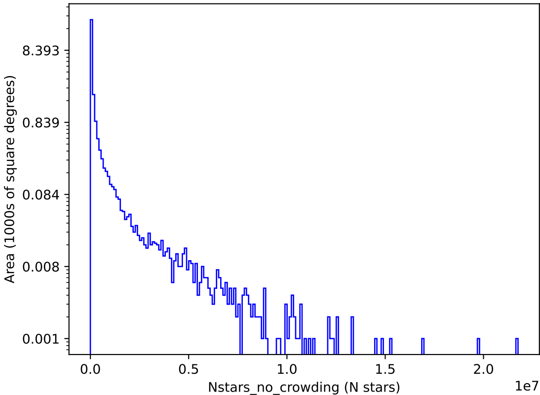
reweight_bulge_v3.3_10yrs r: Nstars_no_crowding
